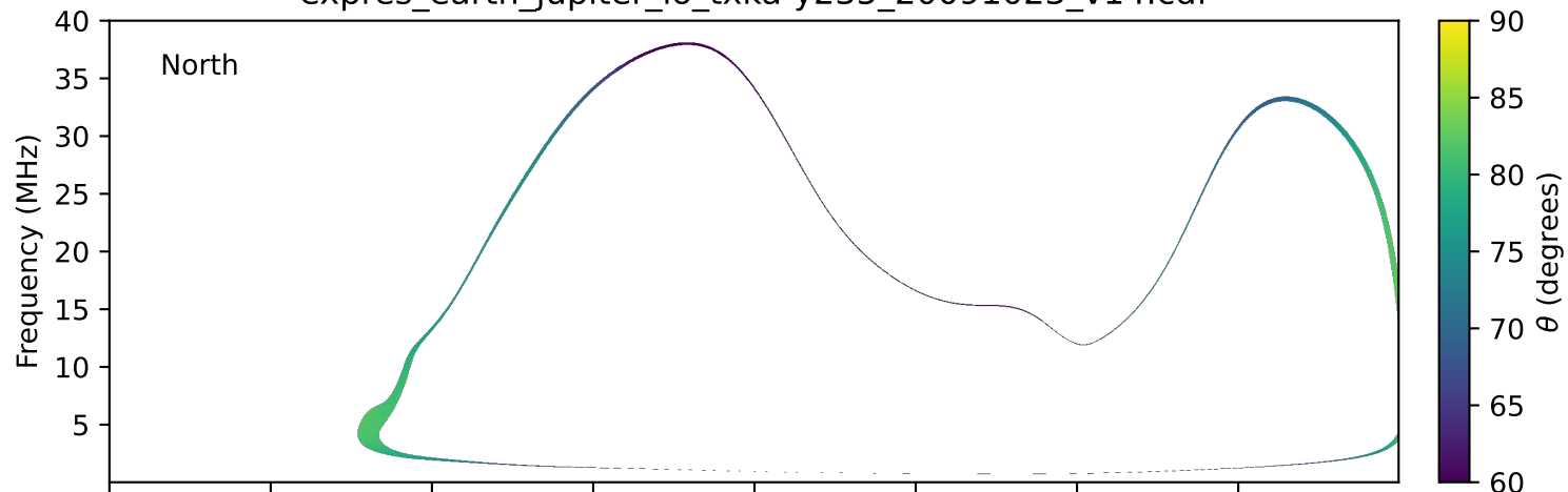
expres_earth_jupiter_io_txka-y235_20091023_v14.cdf
