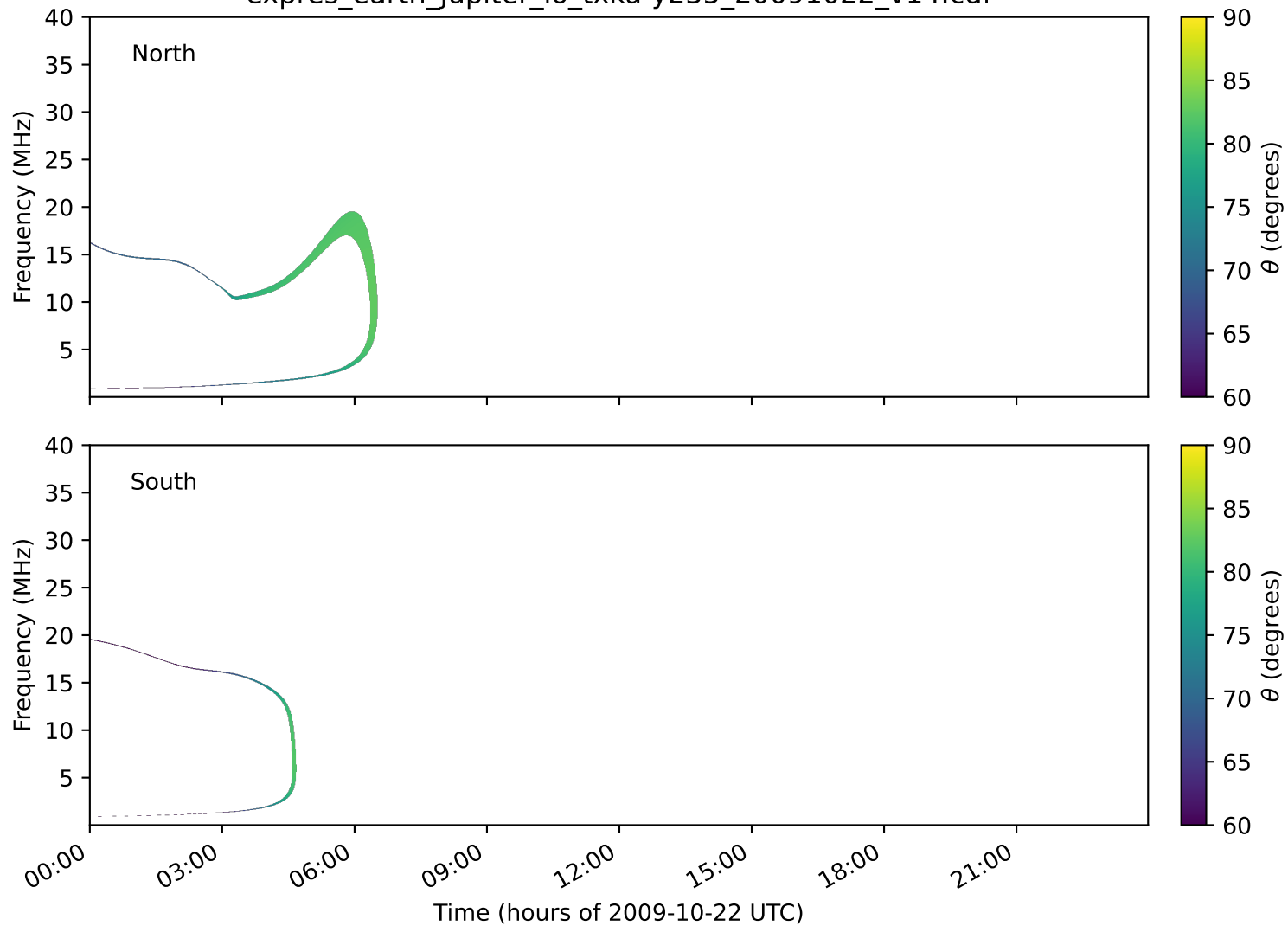
expres_earth_jupiter_io_txka-y235_20091022_v14.cdf
