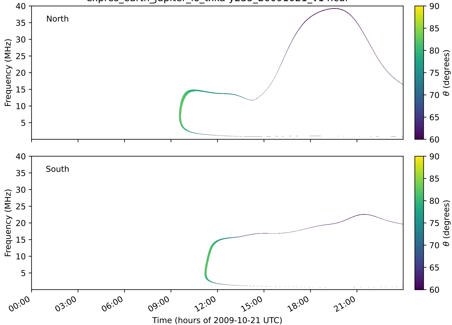
expres_earth_jupiter_io_txka-y235_20091021_v14.cdf
