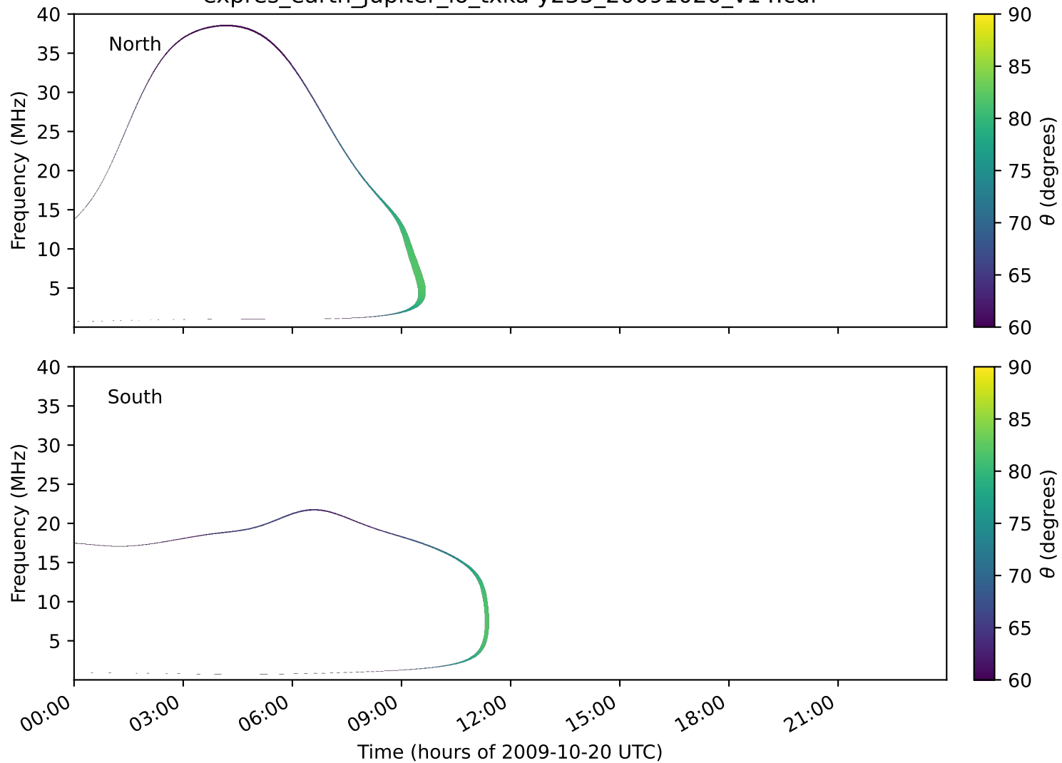
expres_earth_jupiter_io_txka-y235_20091020_v14.cdf
