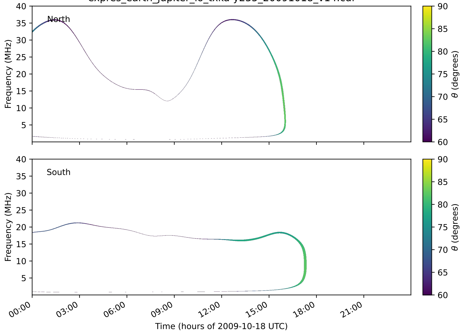
expres_earth_jupiter_io_txka-y235_20091018_v14.cdf
