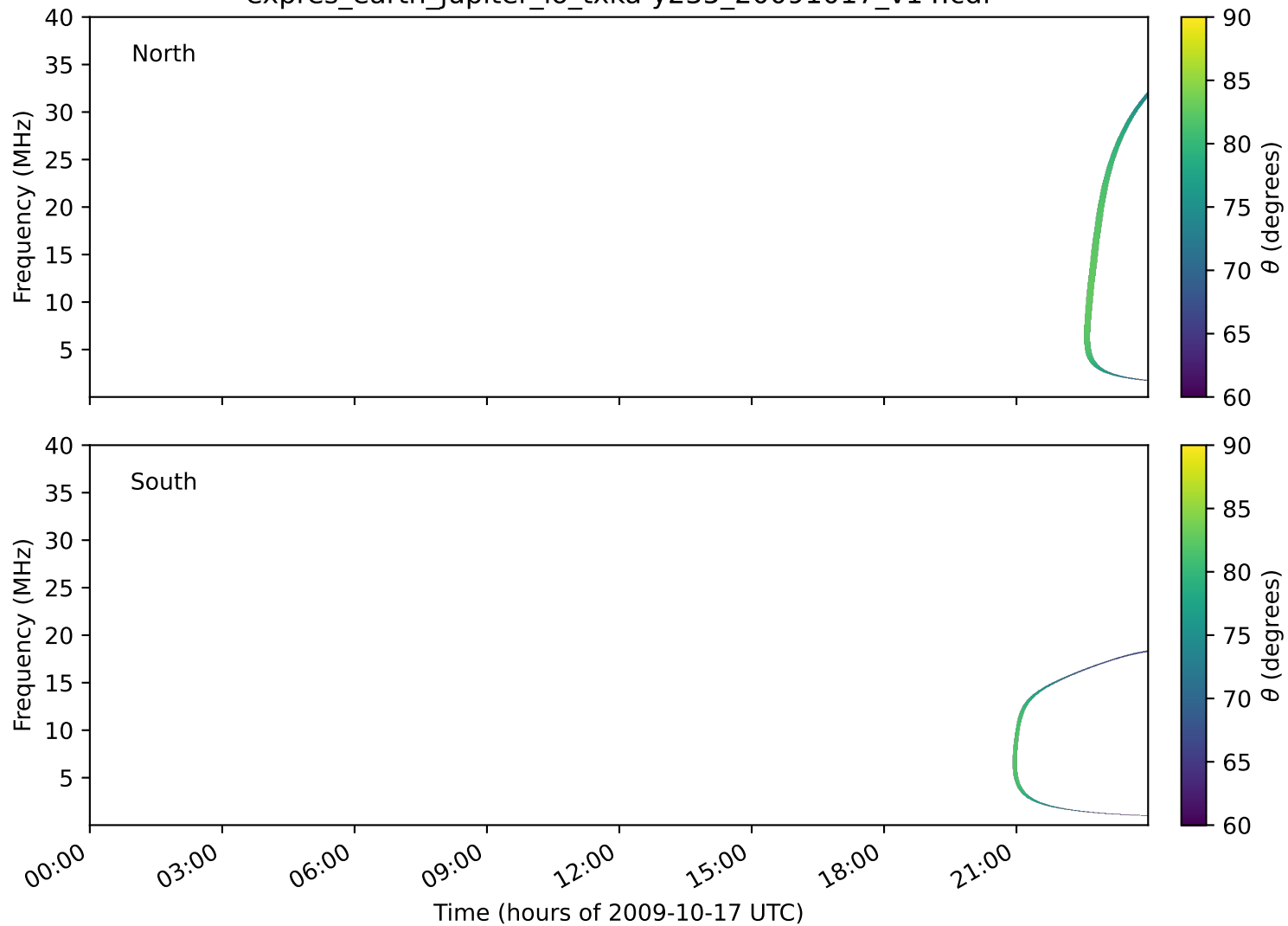
expres_earth_jupiter_io_txka-y235_20091017_v14.cdf
