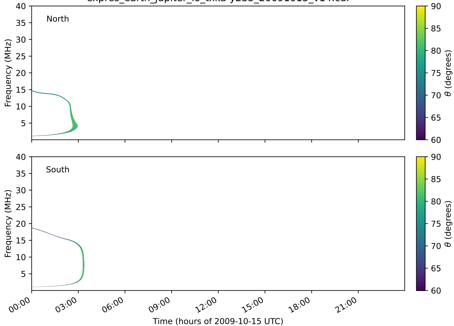
expres_earth_jupiter_io_txka-y235_20091015_v14.cdf
