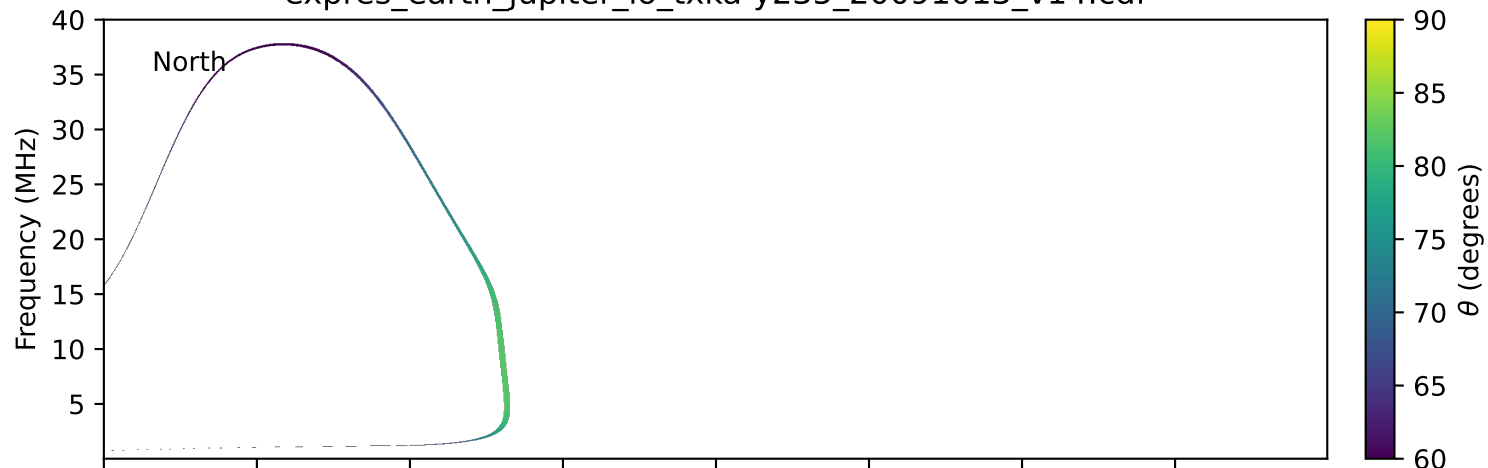
expres_earth_jupiter_io_txka-y235_20091013_v14.cdf
