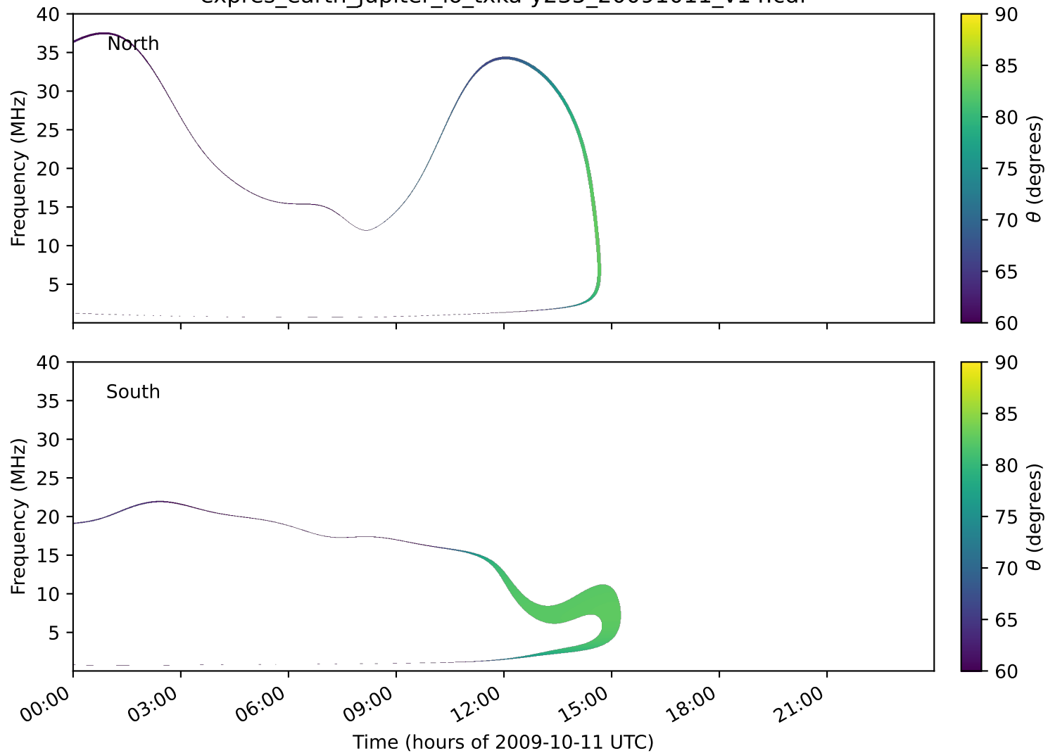
expres_earth_jupiter_io_txka-y235_20091011_v14.cdf
