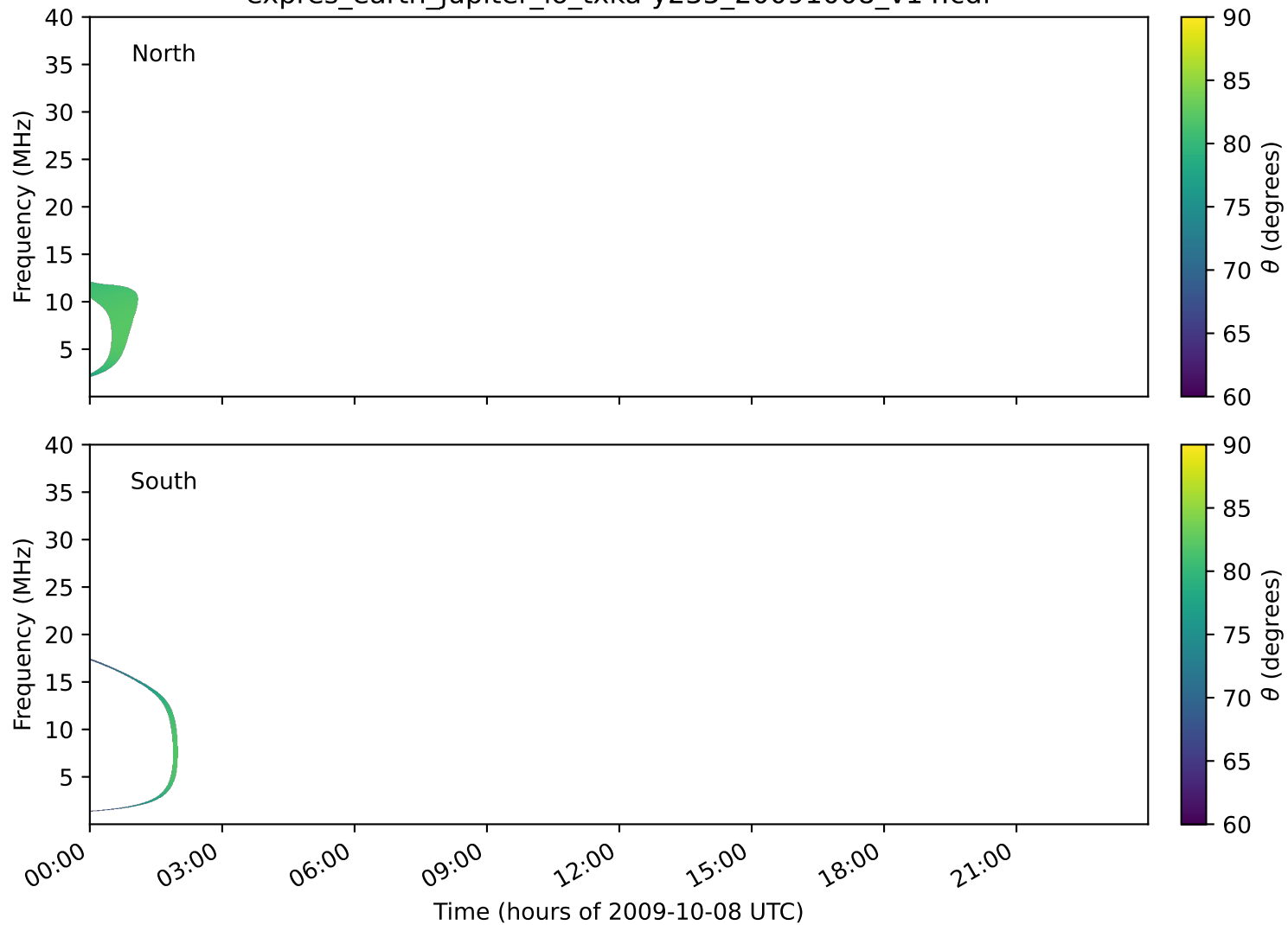
expres_earth_jupiter_io_txka-y235_20091008_v14.cdf
