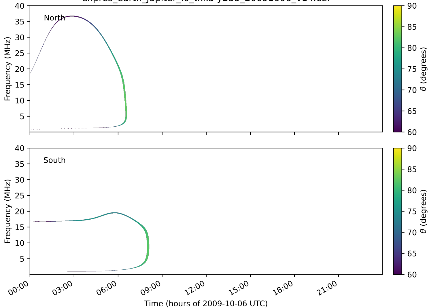
expres_earth_jupiter_io_txka-y235_20091006_v14.cdf
