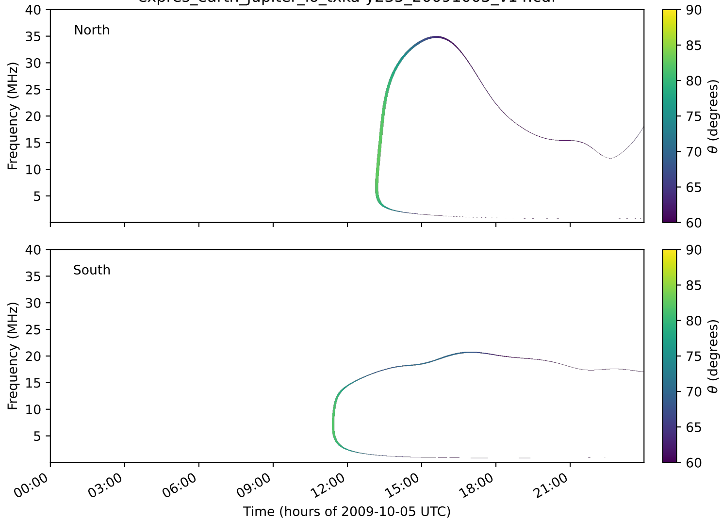
expres_earth_jupiter_io_txka-y235_20091005_v14.cdf
