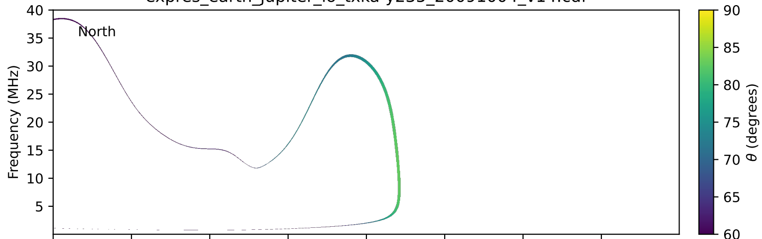
expres_earth_jupiter_io_txka-y235_20091004_v14.cdf
