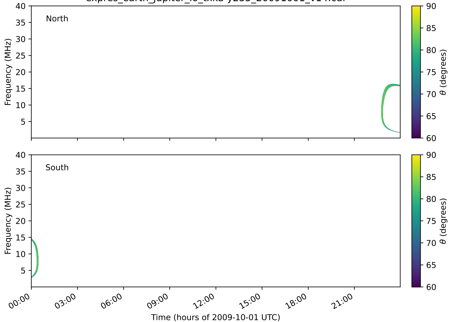
expres_earth_jupiter_io_txka-y235_20091001_v14.cdf
