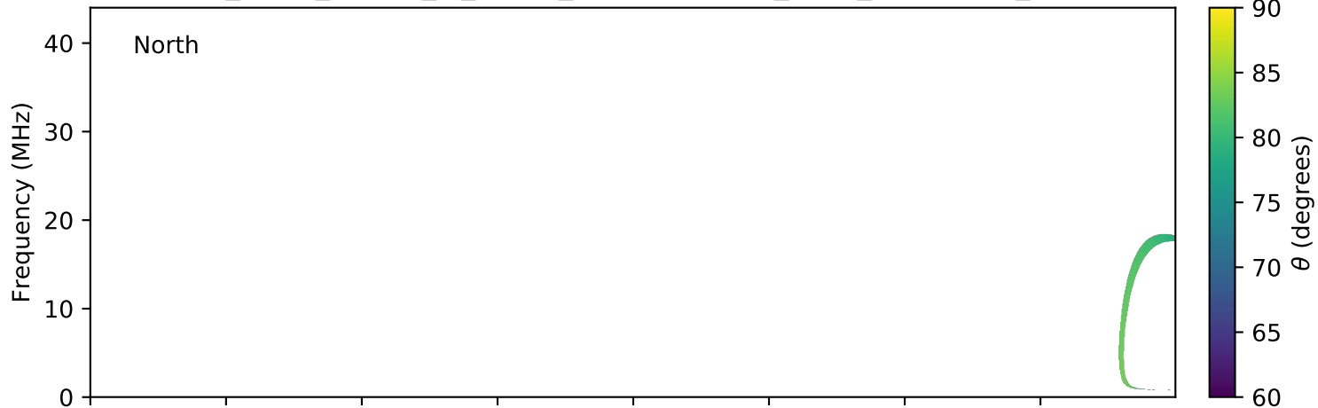
expres_earth_jupiter_io_jrm09_lossc-wid1deg_3kev_20091001_v01.cdf
