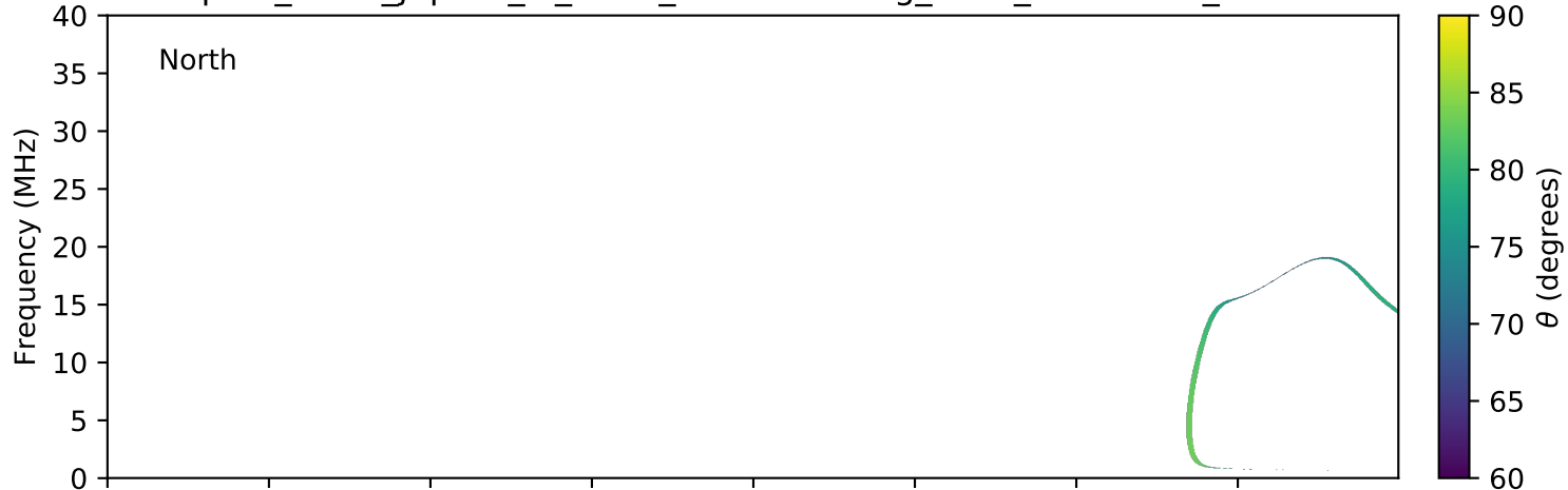
expres_earth_jupiter_io_isaac_lossc-wid1deg_3kev_20091017_v01.cdf
