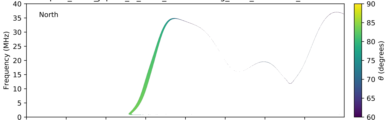
expres_earth_jupiter_io_isaac_lossc-wid1deg_3kev_20091014_v01.cdf
