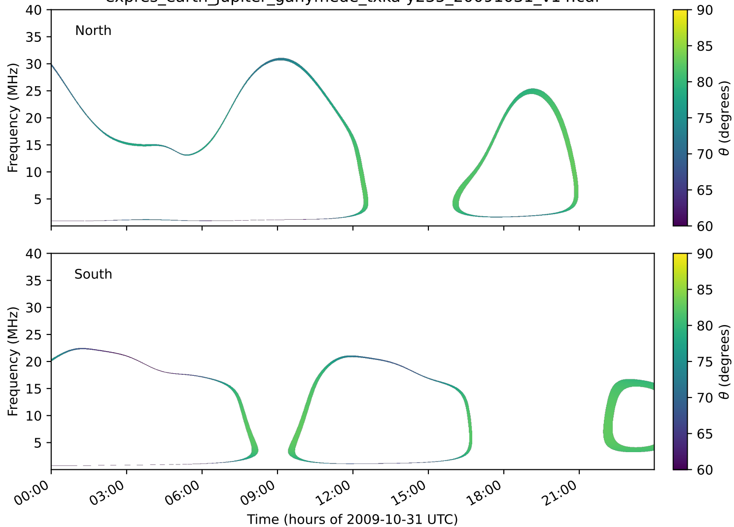
expres_earth_jupiter_ganymede_txka-y235_20091031_v14.cdf
