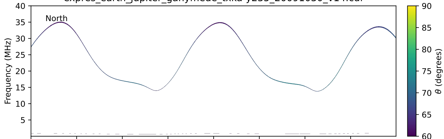
expres_earth_jupiter_ganymede_txka-y235_20091030_v14.cdf
