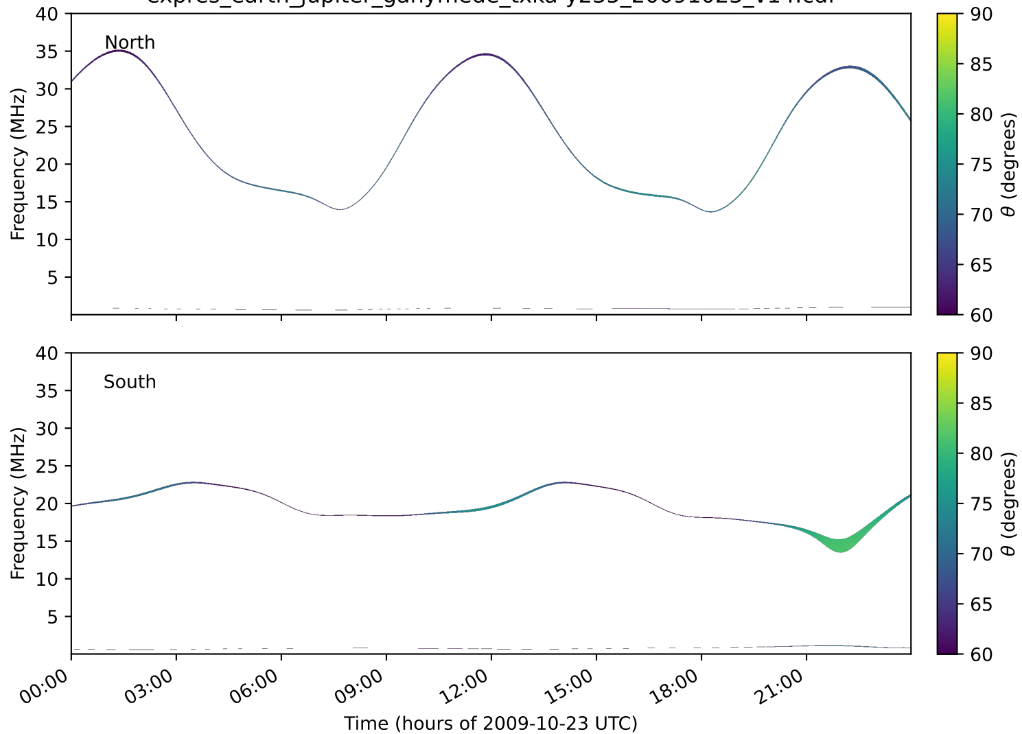
expres_earth_jupiter_ganymede_txka-y235_20091023_v14.cdf
