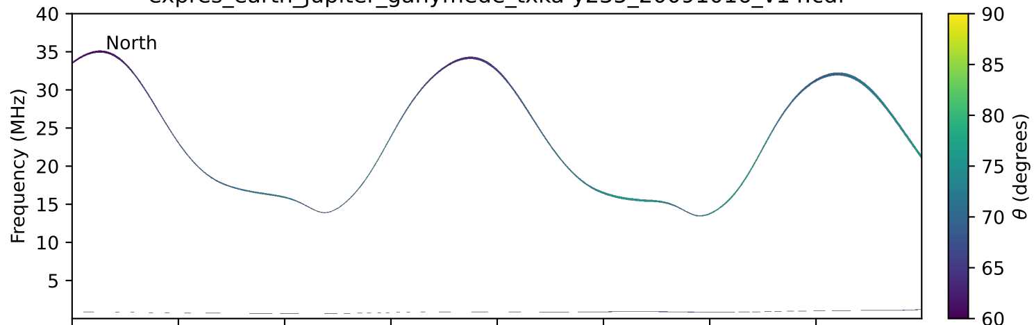
expres_earth_jupiter_ganymede_txka-y235_20091016_v14.cdf
