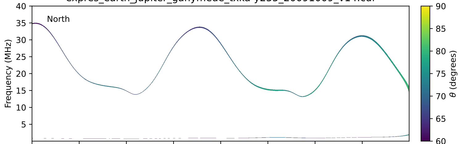
expres_earth_jupiter_ganymede_txka-y235_20091009_v14.cdf
