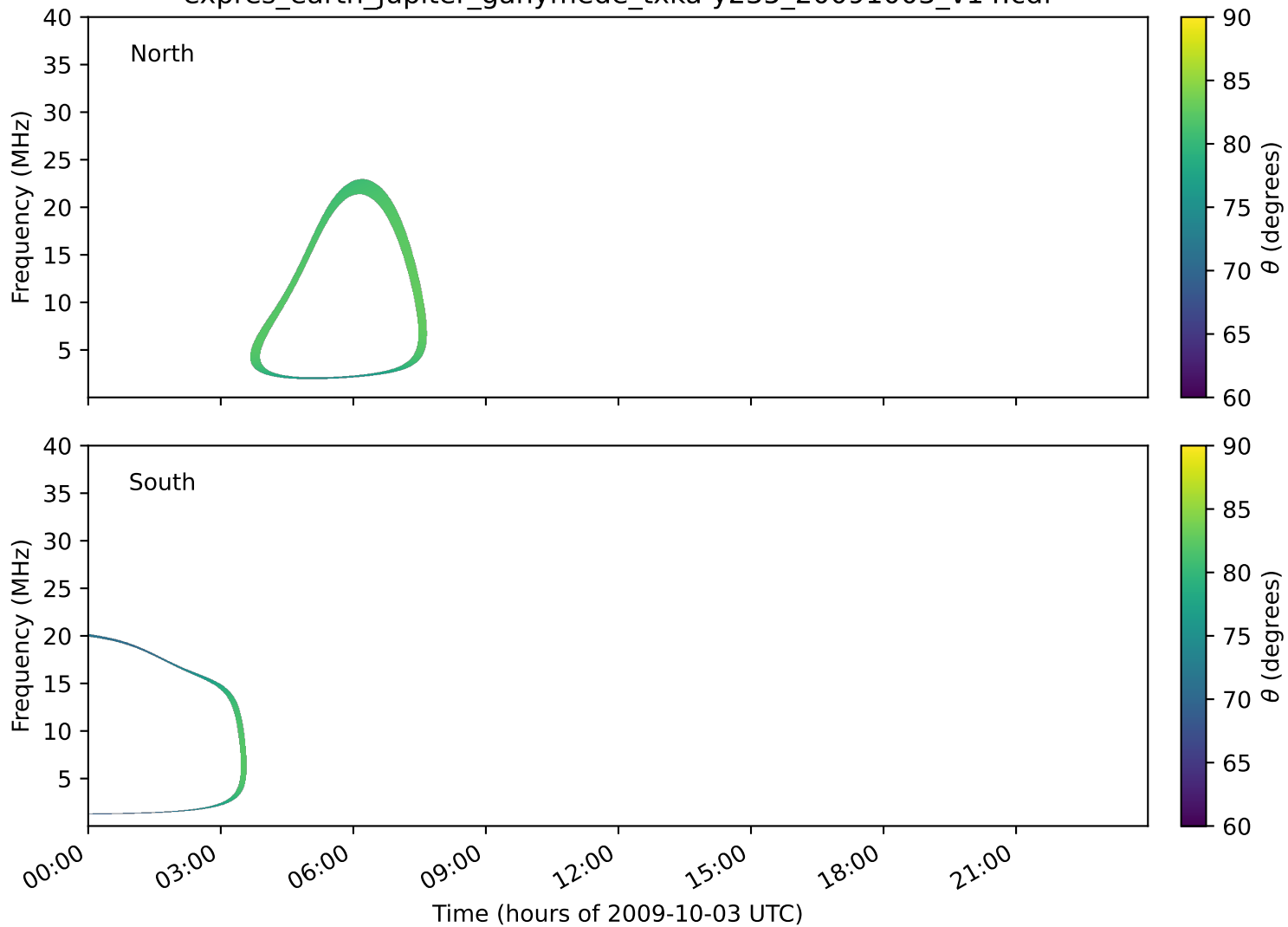
expres_earth_jupiter_ganymede_txka-y235_20091003_v14.cdf
