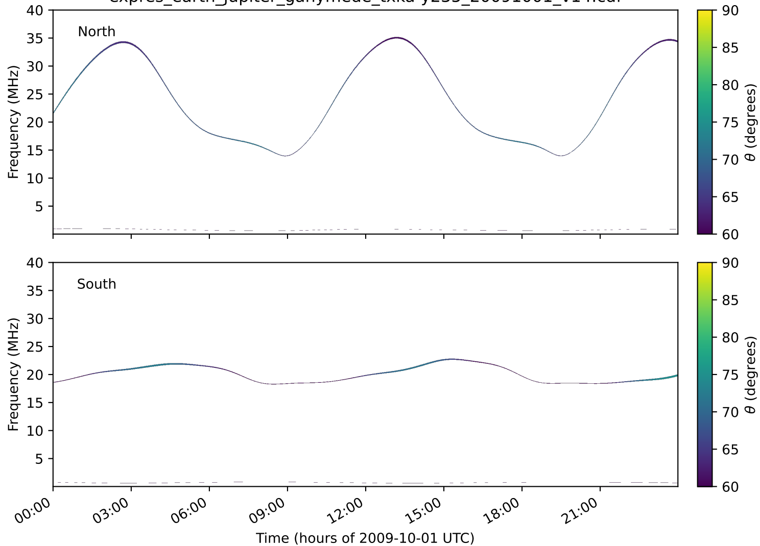
expres_earth_jupiter_ganymede_txka-y235_20091001_v14.cdf
