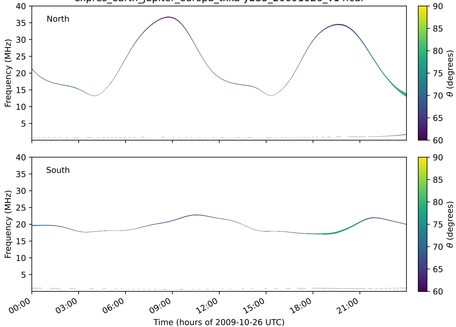
expres_earth_jupiter_europa_txka-y235_20091026_v14.cdf
