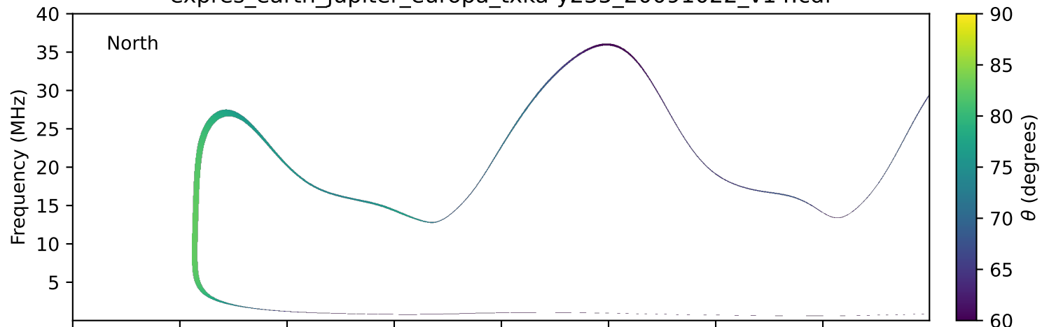
expres_earth_jupiter_europa_txka-y235_20091022_v14.cdf
