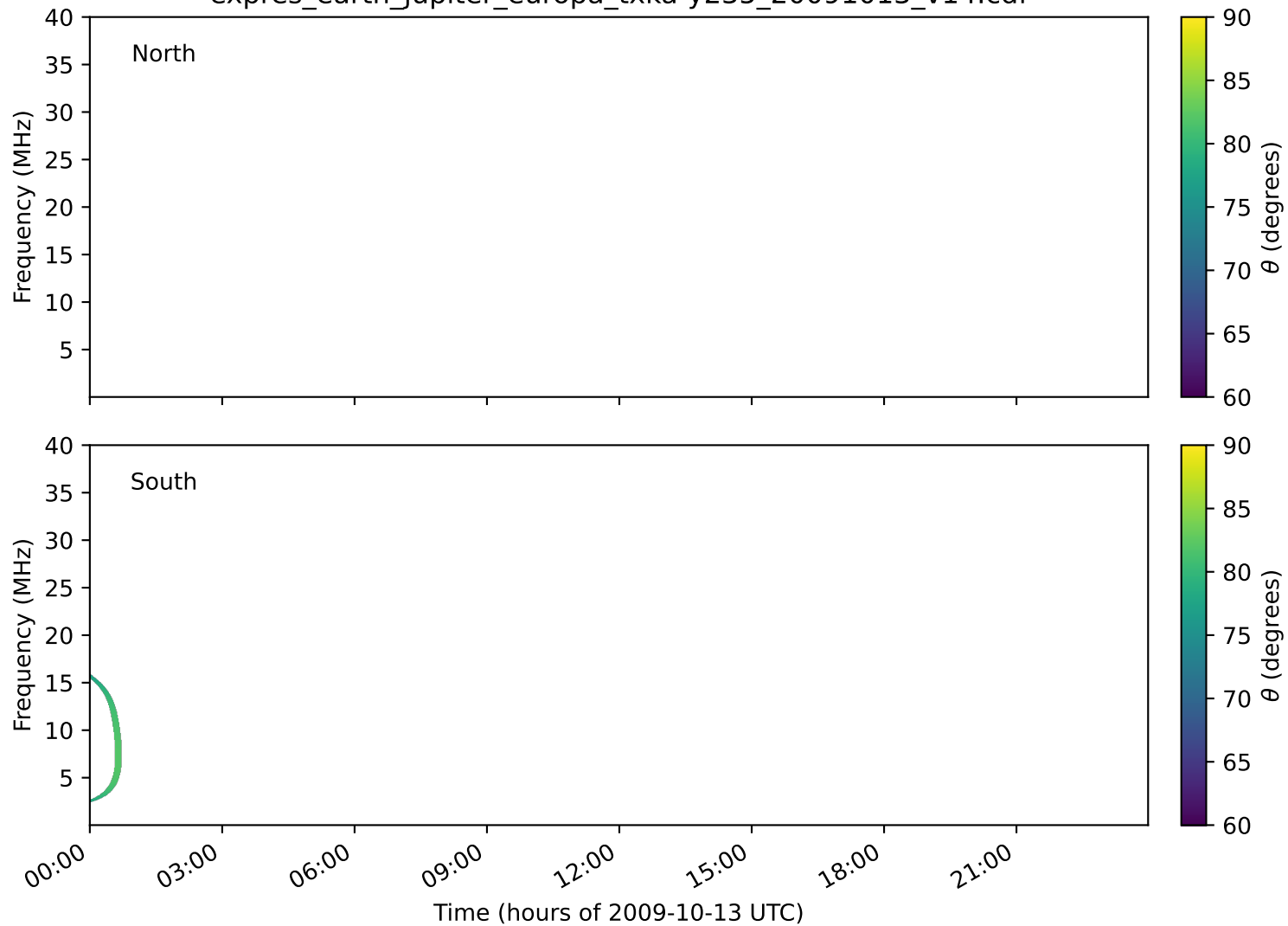
expres_earth_jupiter_europa_txka-y235_20091013_v14.cdf
