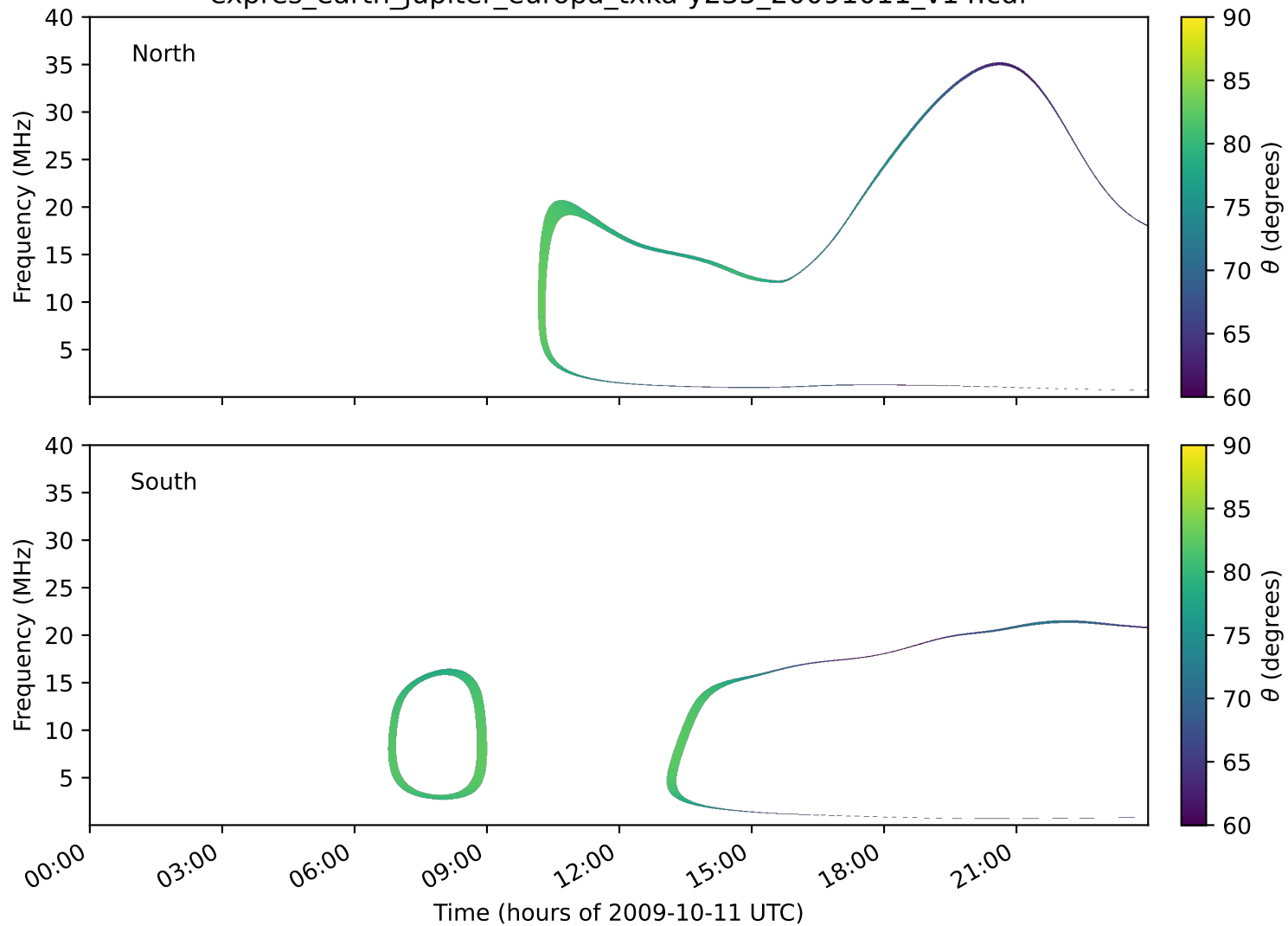
expres_earth_jupiter_europa_txka-y235_20091011_v14.cdf
