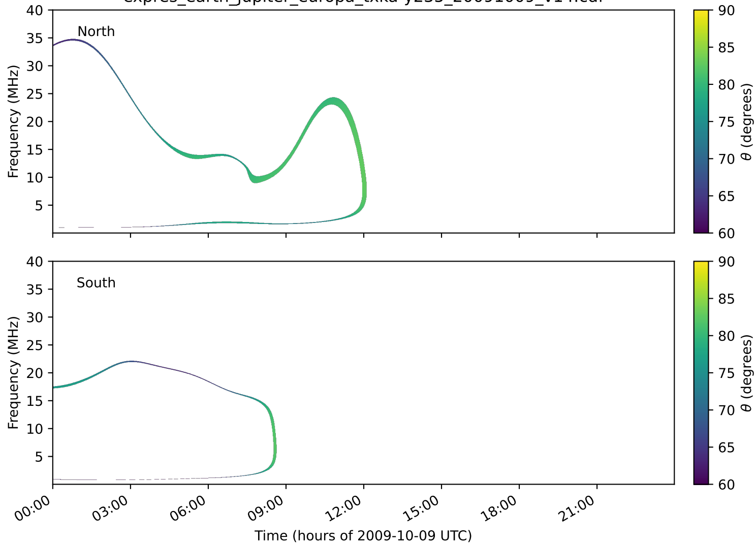
expres_earth_jupiter_europa_txka-y235_20091009_v14.cdf
