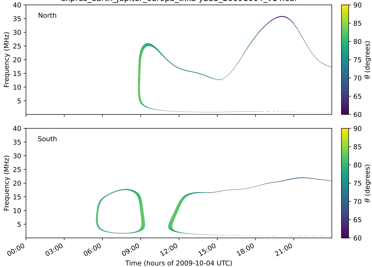
expres_earth_jupiter_europa_txka-y235_20091004_v14.cdf
