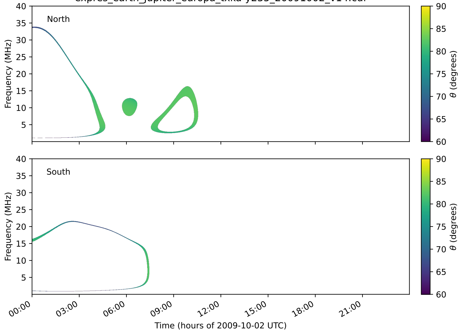
expres_earth_jupiter_europa_txka-y235_20091002_v14.cdf
