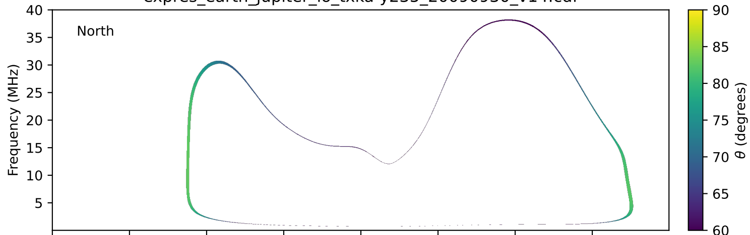
expres_earth_jupiter_io_txka-y235_20090930_v14.cdf
