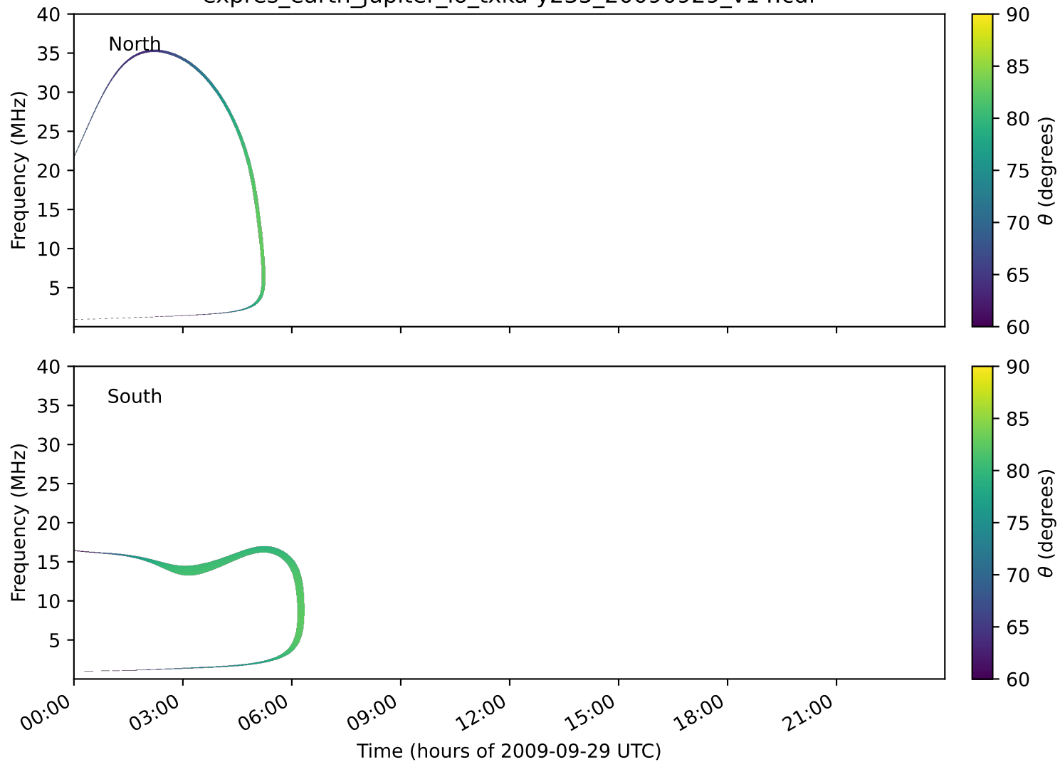
expres_earth_jupiter_io_txka-y235_20090929_v14.cdf
