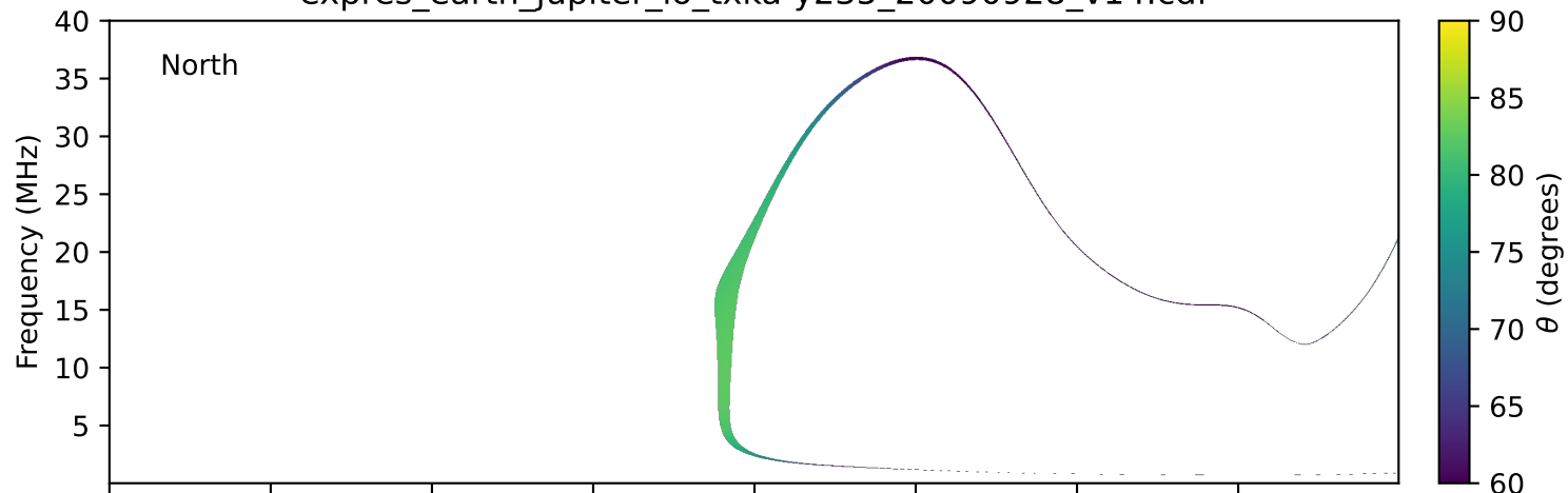
expres_earth_jupiter_io_txka-y235_20090928_v14.cdf
