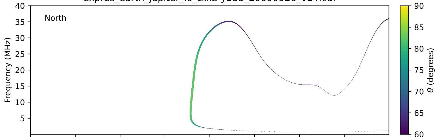
expres_earth_jupiter_io_txka-y235_20090926_v14.cdf
