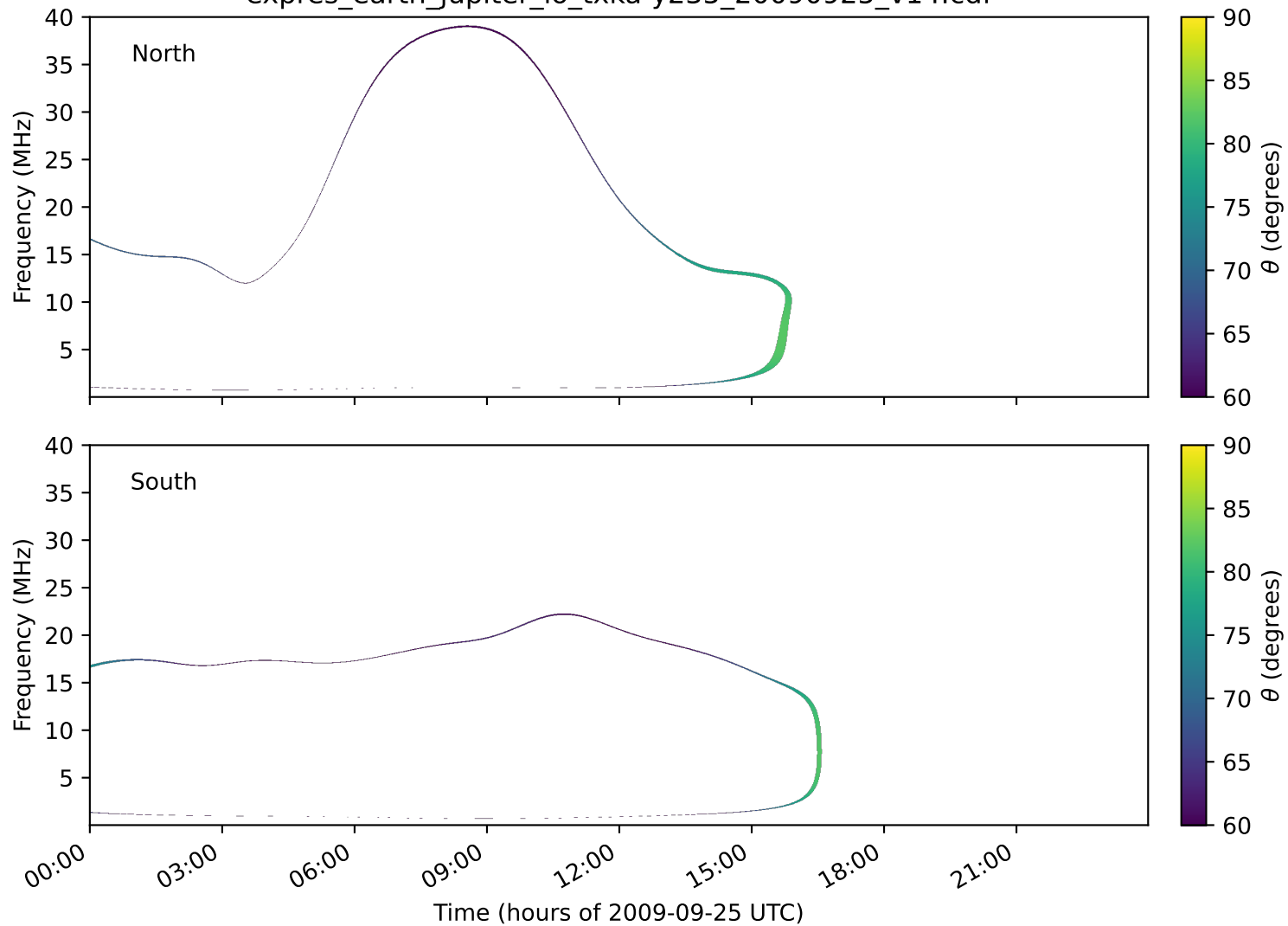
expres_earth_jupiter_io_txka-y235_20090925_v14.cdf
