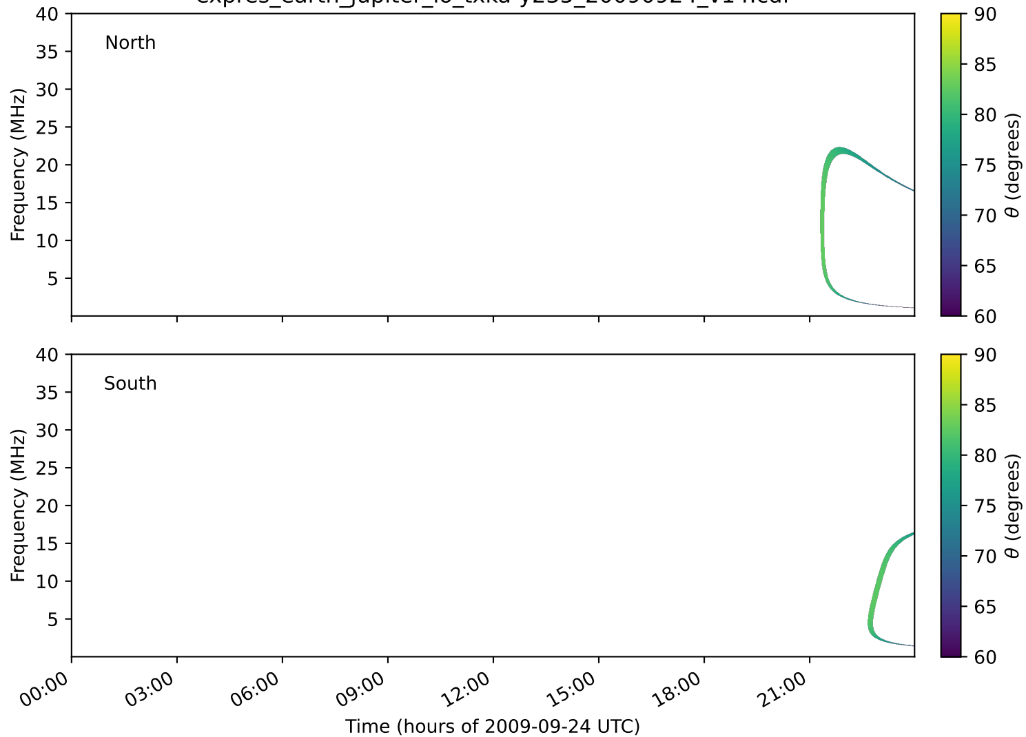
expres_earth_jupiter_io_txka-y235_20090924_v14.cdf
