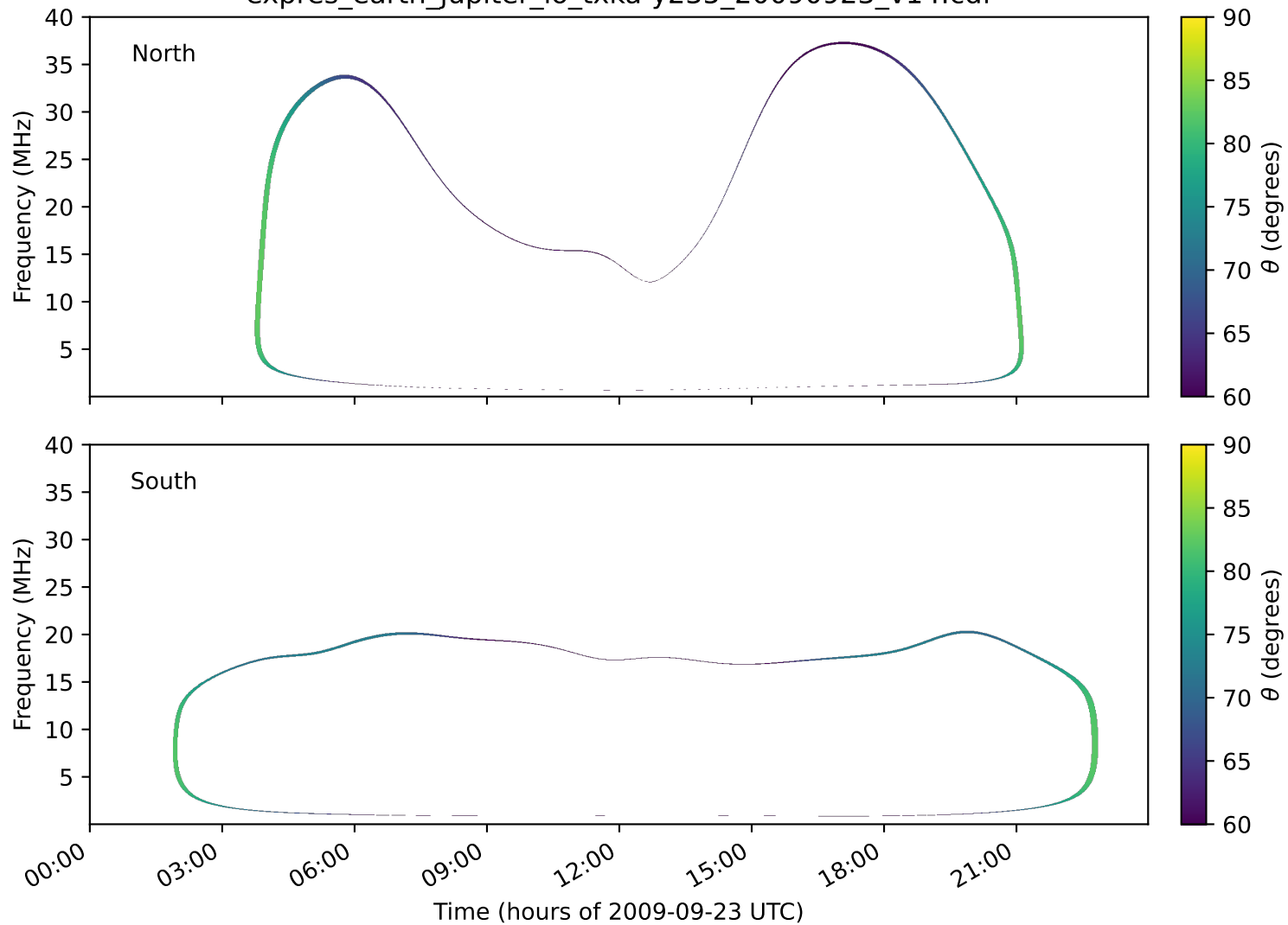
expres_earth_jupiter_io_txka-y235_20090923_v14.cdf
