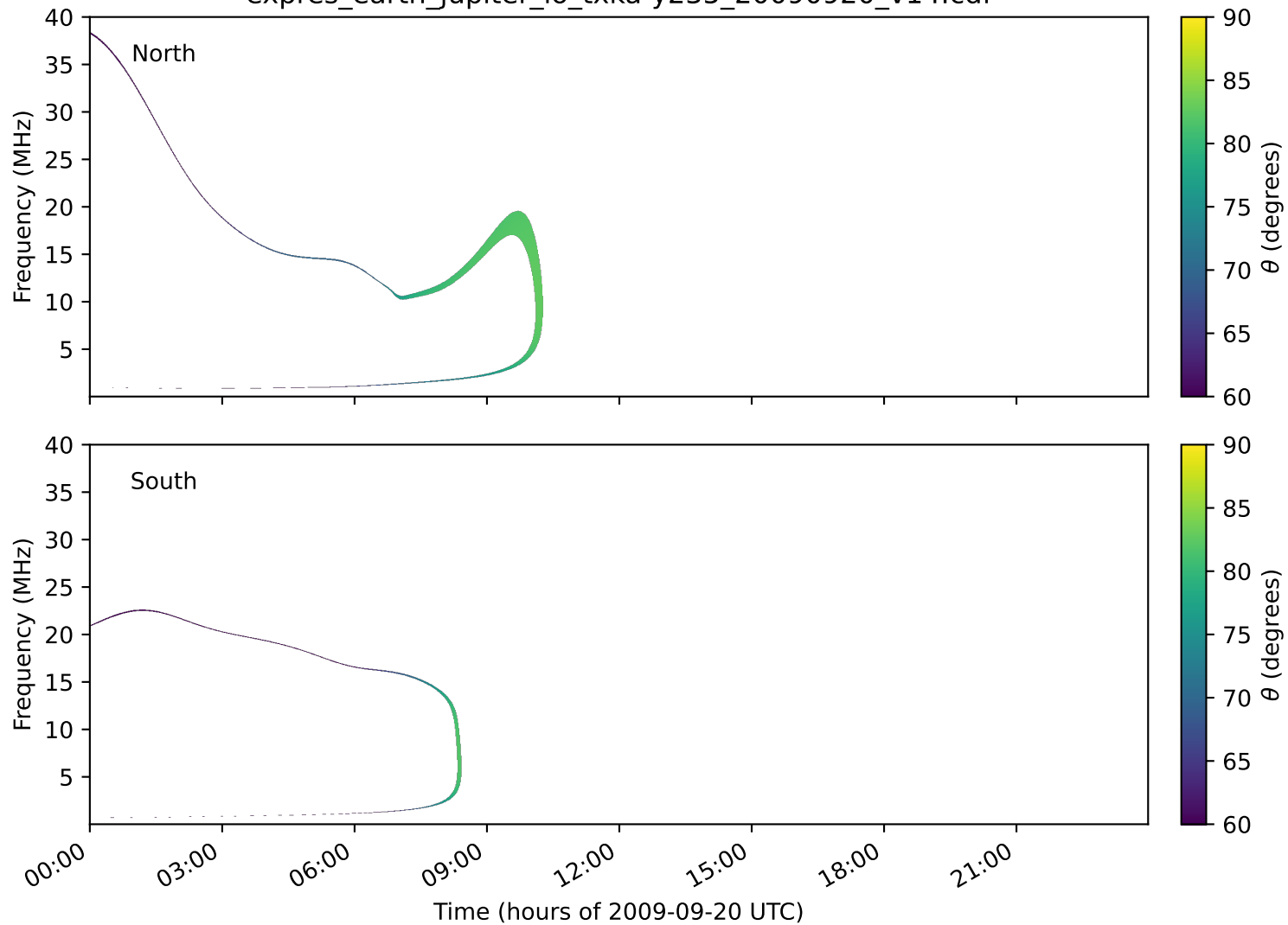
expres_earth_jupiter_io_txka-y235_20090920_v14.cdf
