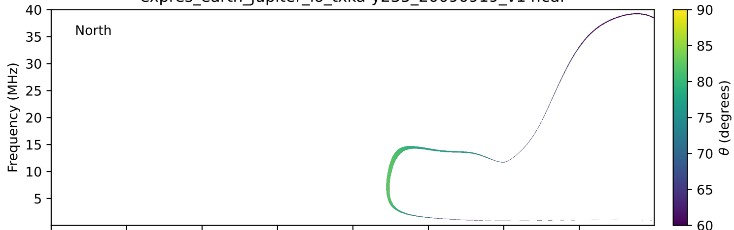
expres_earth_jupiter_io_txka-y235_20090919_v14.cdf
