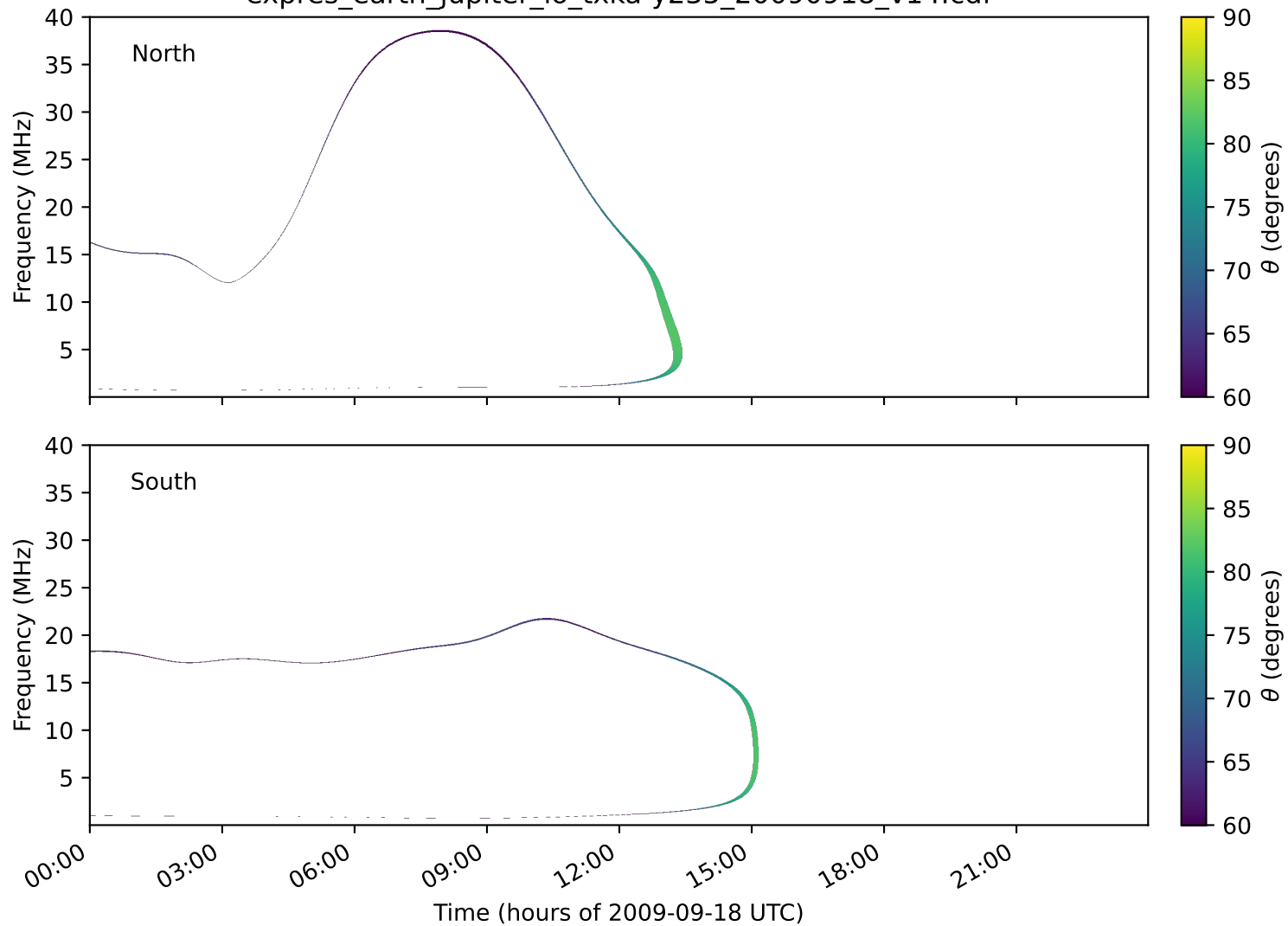
expres_earth_jupiter_io_txka-y235_20090918_v14.cdf
