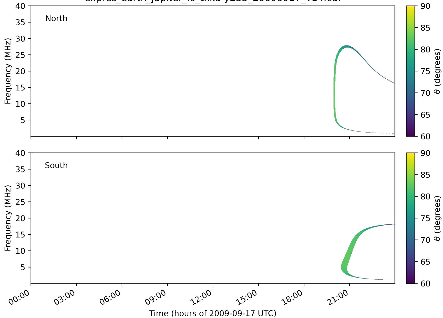
expres_earth_jupiter_io_txka-y235_20090917_v14.cdf
