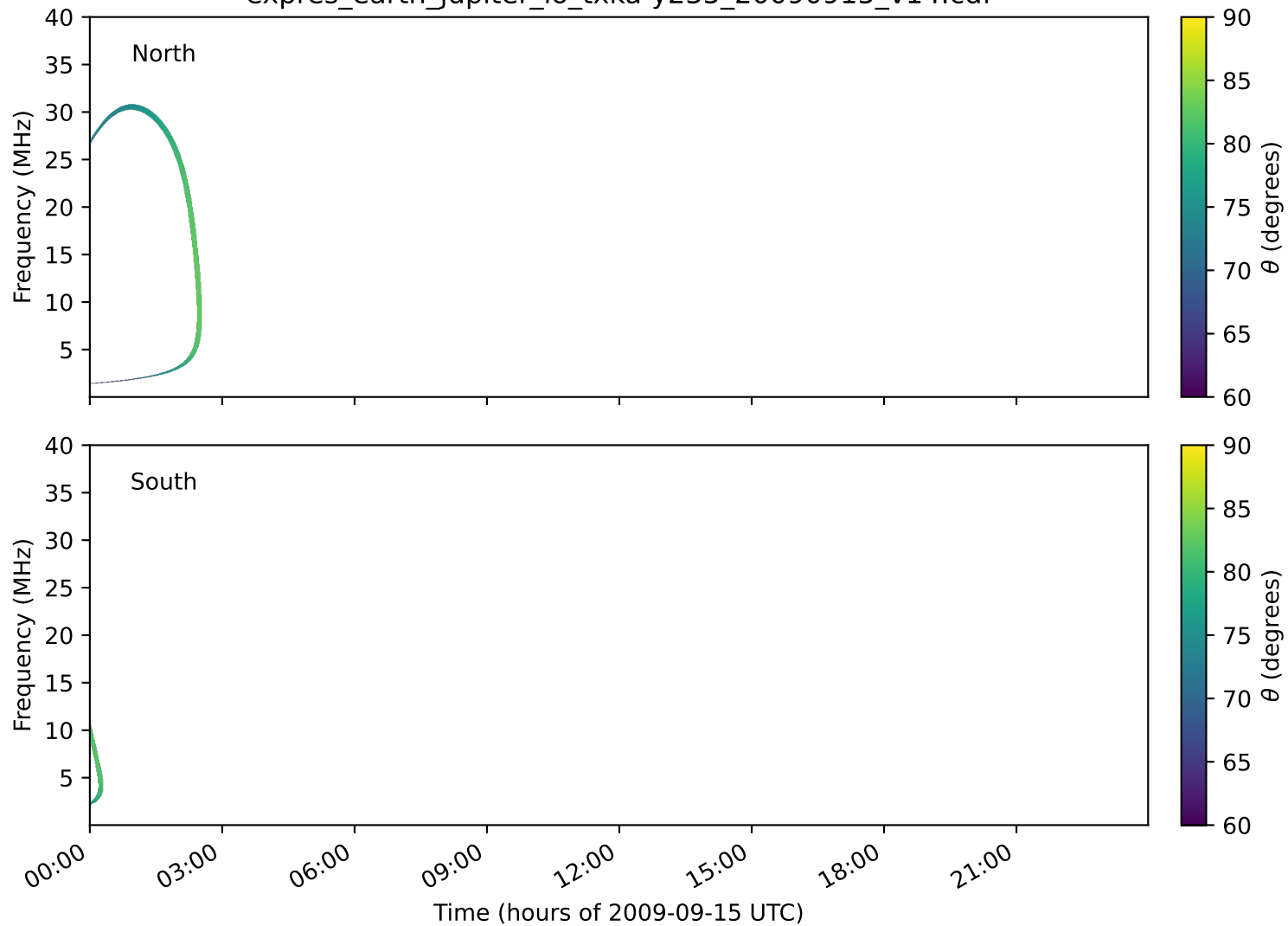
expres_earth_jupiter_io_txka-y235_20090915_v14.cdf
