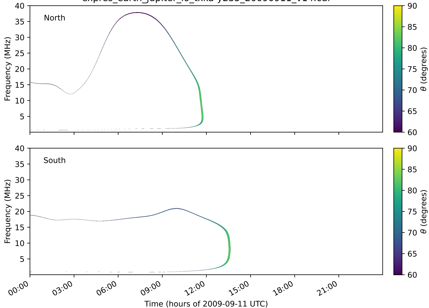
expres_earth_jupiter_io_txka-y235_20090911_v14.cdf
