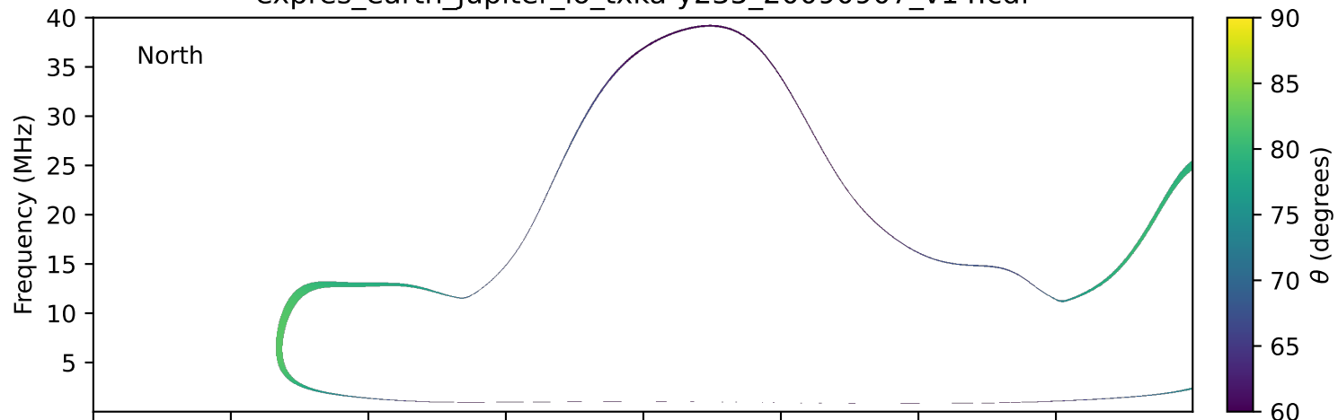
expres_earth_jupiter_io_txka-y235_20090907_v14.cdf
