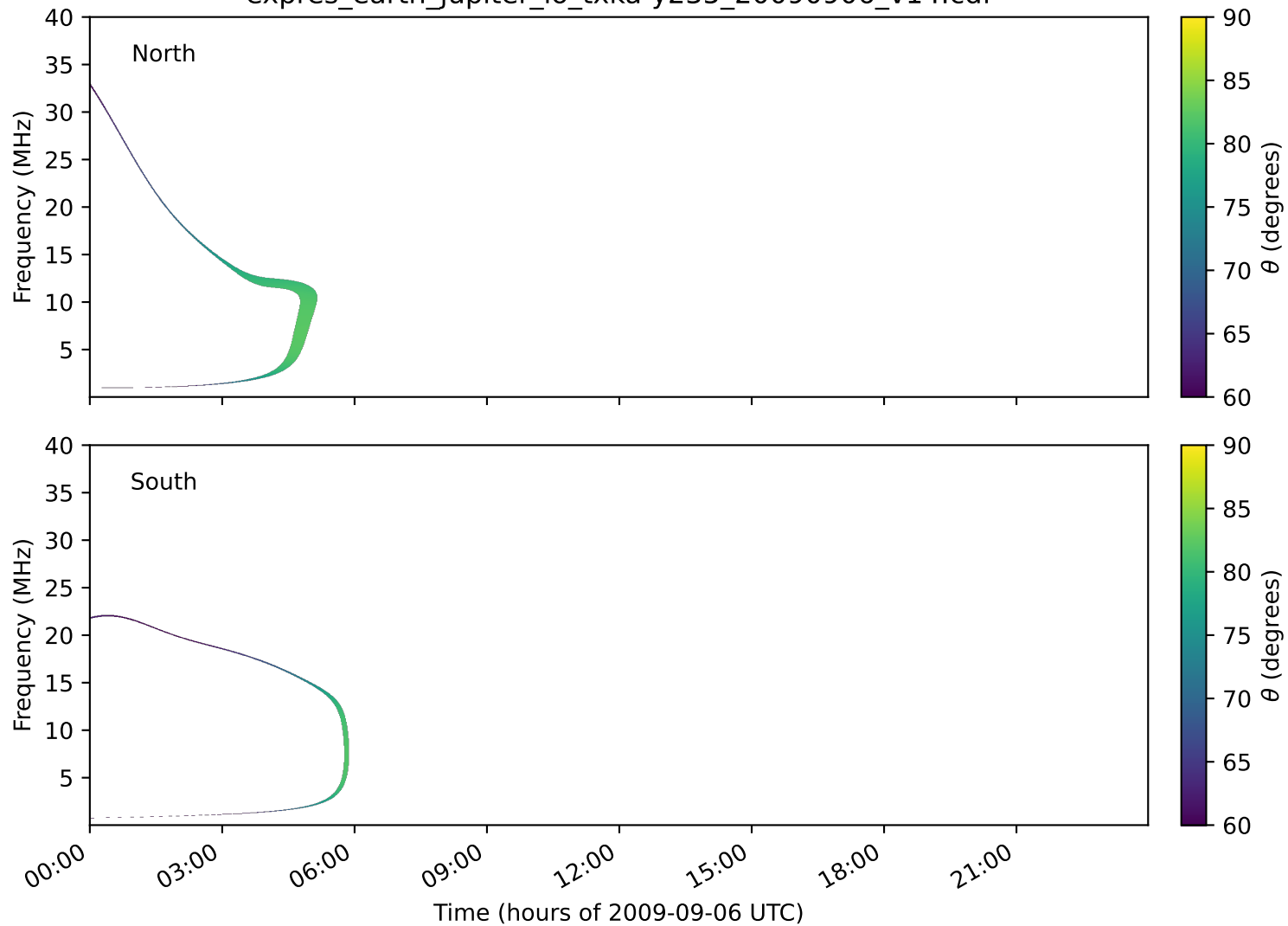
expres_earth_jupiter_io_txka-y235_20090906_v14.cdf
