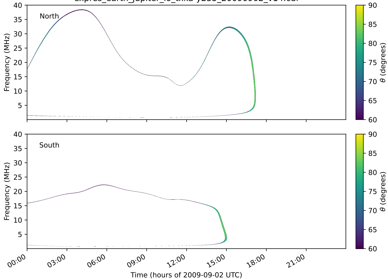
expres_earth_jupiter_io_txka-y235_20090902_v14.cdf
