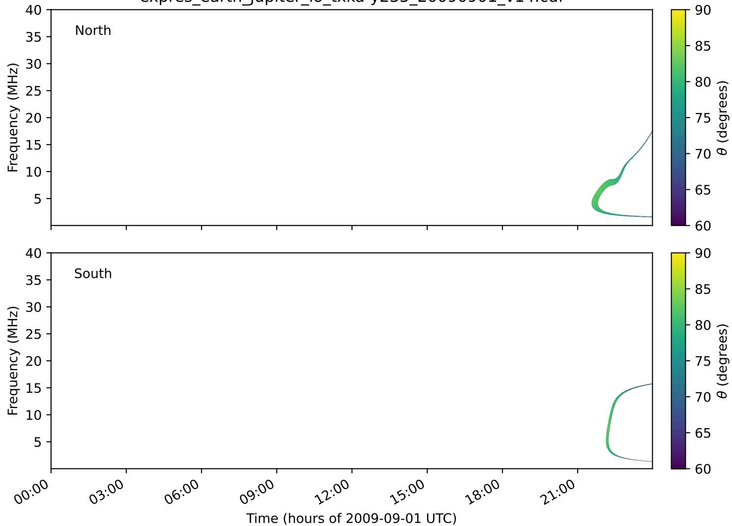
expres_earth_jupiter_io_txka-y235_20090901_v14.cdf
