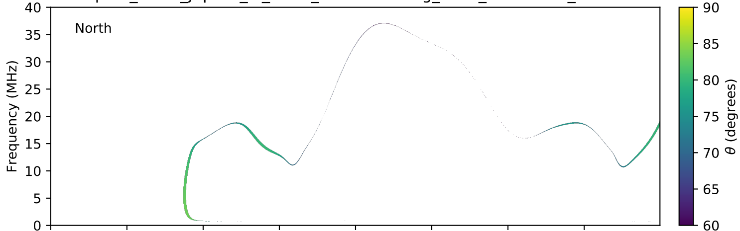
expres_earth_jupiter_io_isaac_lossc-wid1deg_3kev_20090914_v01.cdf
