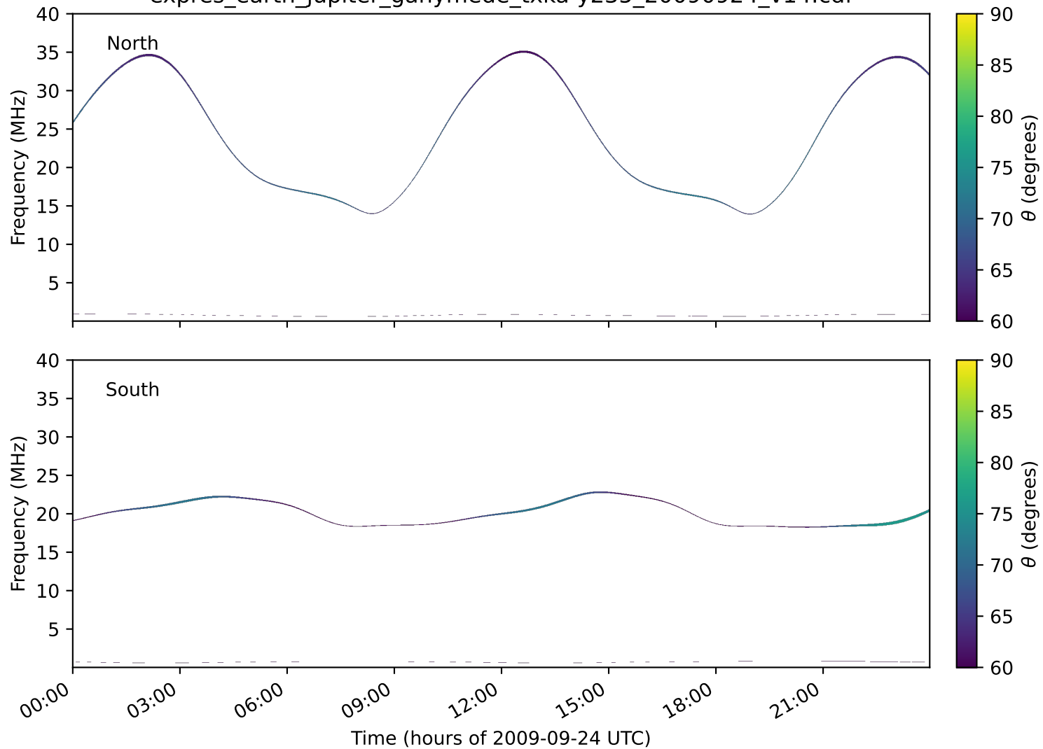
expres_earth_jupiter_ganymede_txka-y235_20090924_v14.cdf
